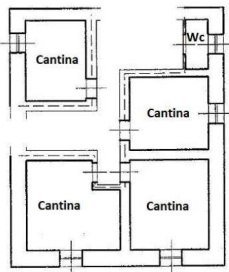
Piano TERRA H = 2.23
