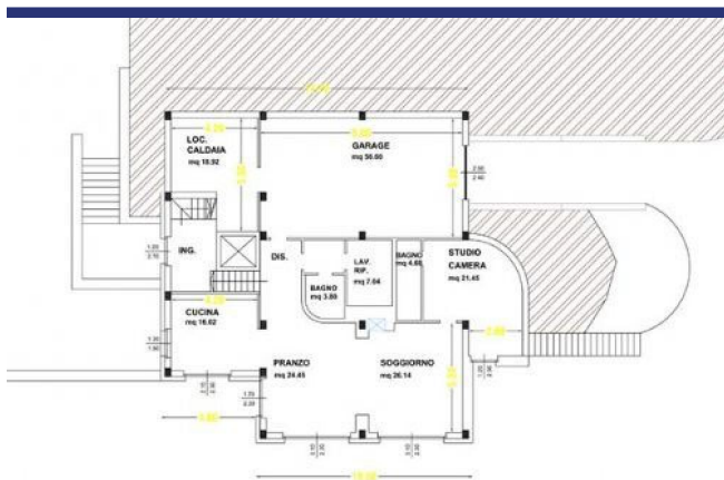
PIANO TERRA
