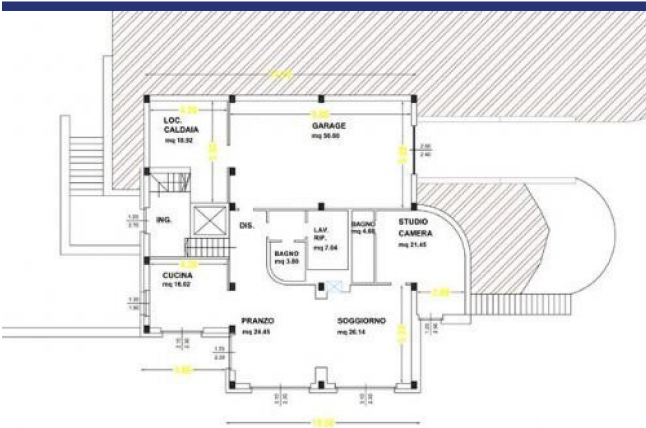
PIANO TERRA
